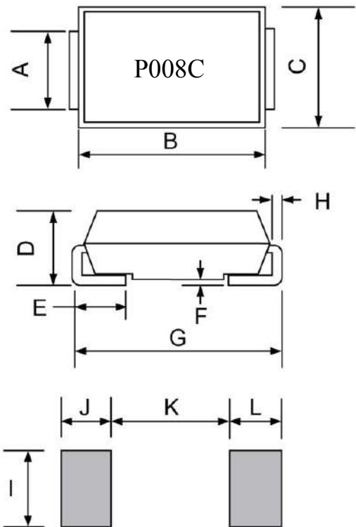
SMB/DO-214AA
