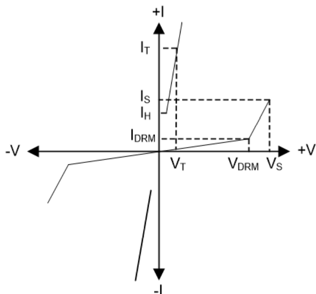
Figure 1.V-I Characteristic
